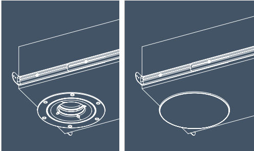
6/8" ROUND GRILLE ADAPTER
